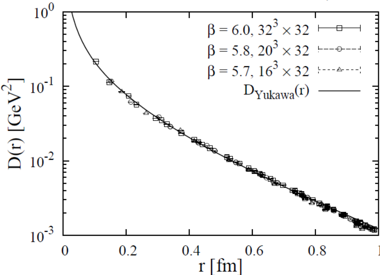
FIG. 7: The Yukawa-type function D_{\text{Yukawa}}(r) = A m e^{-mr} / r (solid line) with m = 0.624 \text{ GeV} and A = 0.237 obtained by the fit analysis at \beta = 6.0 , and the lattice QCD data of the scalar-type gluon propagator D(r) in the Landau gauge at \beta = 5.7, 5.8 , and 6.0 in the range of r = 0.1 \sim 1.0 \text{ fm} . The
