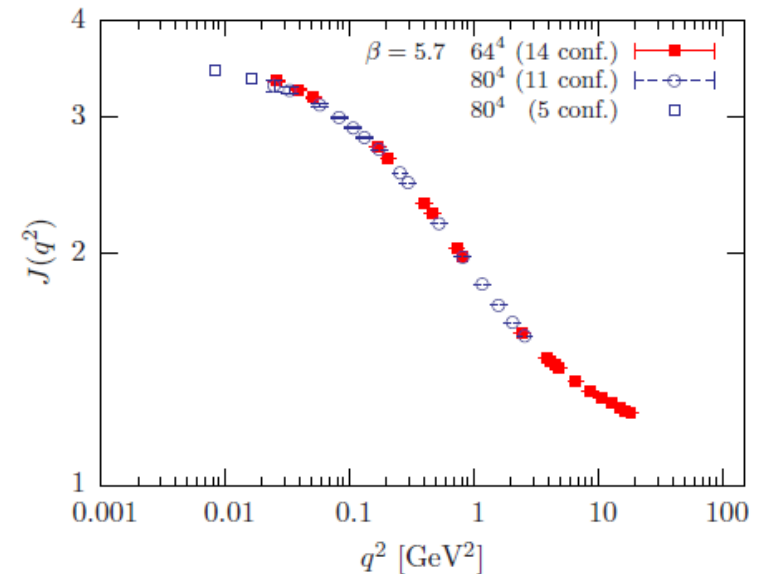
Figure 4: Bare ghost dressing function J(q^2) versus q^2 for L = 64, 80 at \beta = 5.70 . Errors are not shown at the two lowest q^2 (squares).
